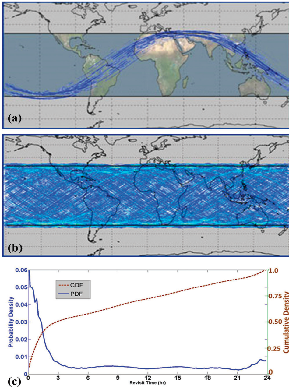
Figure 4: CYGNSS coverage illustration. Each low-Earth orbiting CYGNSS observatory will orbit at an inclination of 35^\circ and is capable of measuring four simultaneous reflections, resulting in 32 wind measurements per second across the Earth. The configuration is optimized for high
