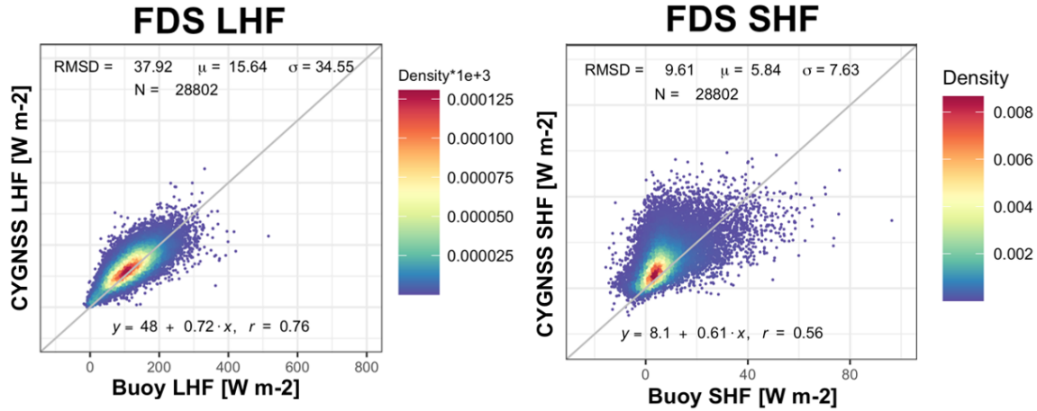
Figure 5: CYGNSS surface heat flux comparisons (y-axis) compared to flux estimates from buoys (x-axis). Left: Latent heat flux. Right: Sensible heat flux.
