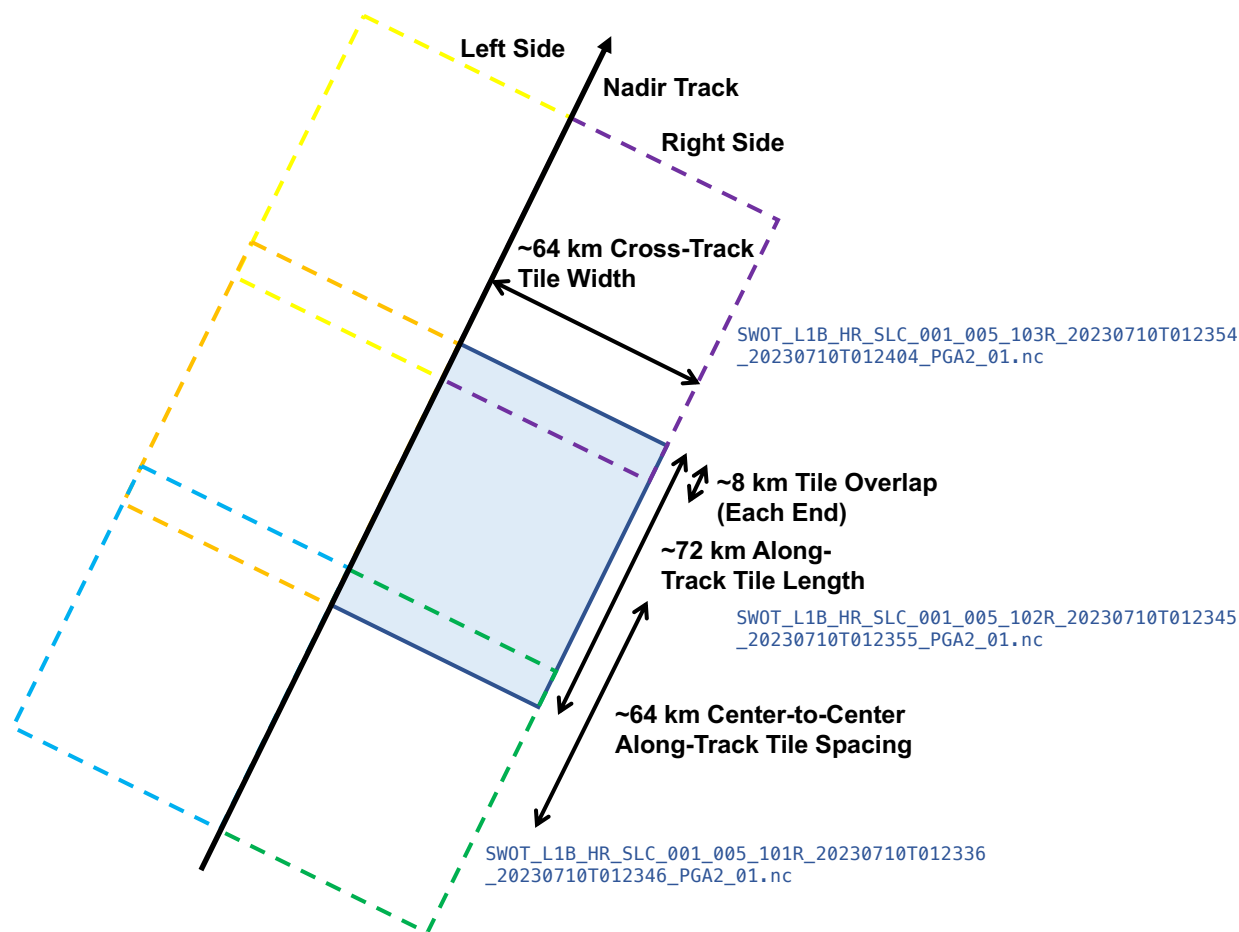
Figure 1. SLC product granulate illustration.
