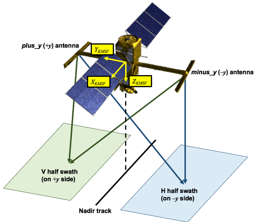
Figure 3. Illustration of the KMSF frame and the polarizations (V and H) of the two KaRIn half swaths. The velocity direction can be along +X_{KMSF} or -X_{KMSF} depending on the yaw state of the spacecraft.
