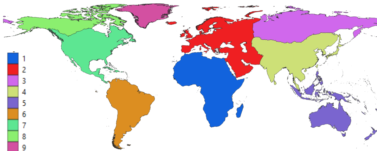
Figure 6. Geographical delineation of continents from HydroBASINS [10].
