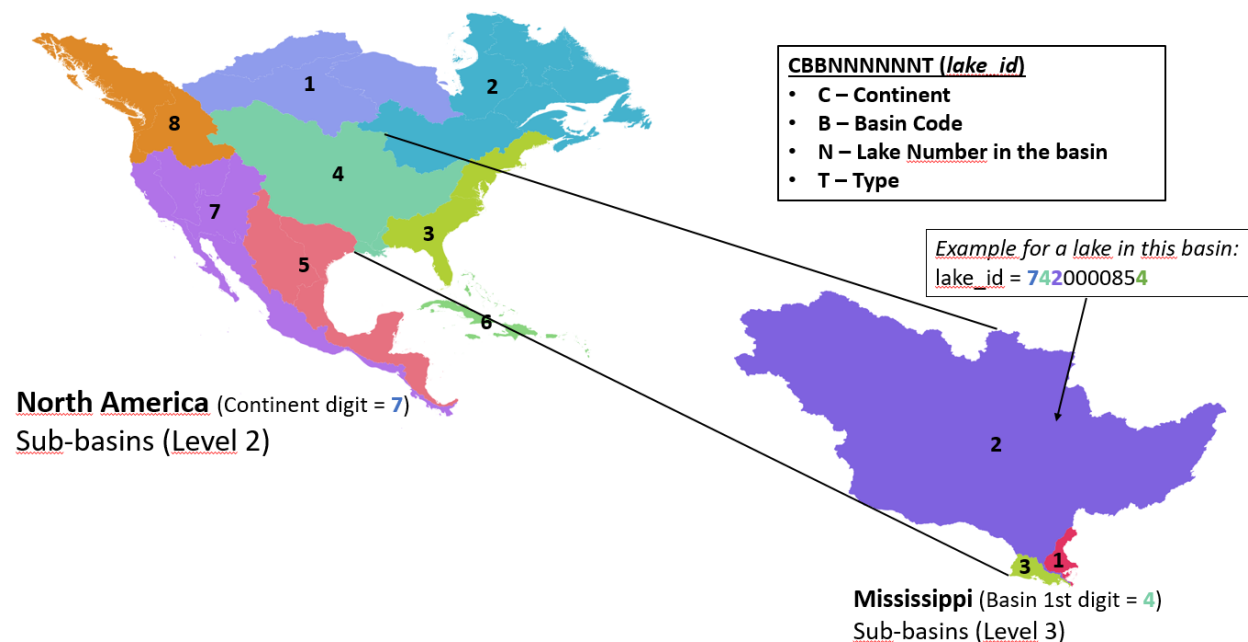
Figure 7. Example of the Pfafstetter basin coding system over North America, limited to the 3 first levels used in the identifiers of the lake products.
