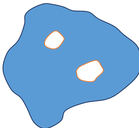
Figure 4. The lake surface (in blue) corresponds to the area comprised between the outer ring (i.e. the lake boundary, in dark blue) and any inner rings (i.e. possible islands, in orange).
