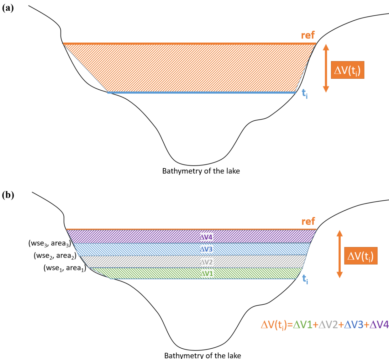
Figure 9. Water volume between the current observation at t_i and the reference state ref , computed with (a) the direct approach and (b) the incremental approach. For the incremental approach, the wse_j and area_j , stored in the PLD, are obtained by a curve fitting a set of observed (wse, area\_total) pairs. Note that, to ease comprehension, measurements are represented as ideal on these figures, i.e. perfectly fitting the bathymetry.
